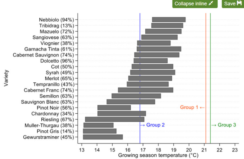
Figure 5. Optimal GST ranges for high-quality winegrape production (shares of world winegrape area under the grey ranges are shown in parentheses on the vertical axis).
